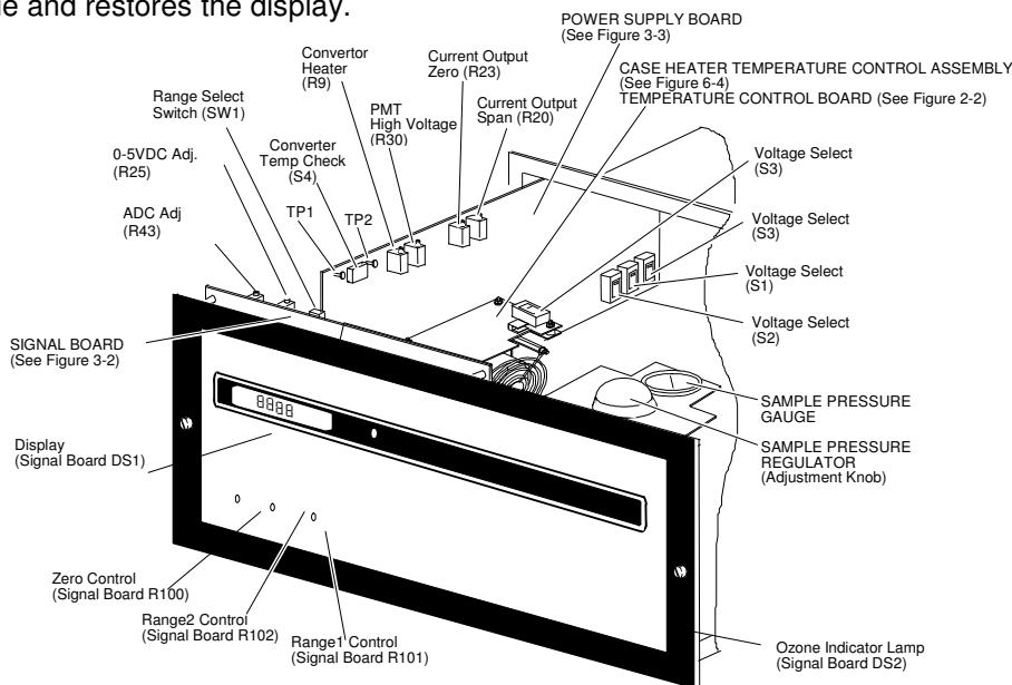
Figure 3-1. Model 951C Controls, Indicators and Adjustments
